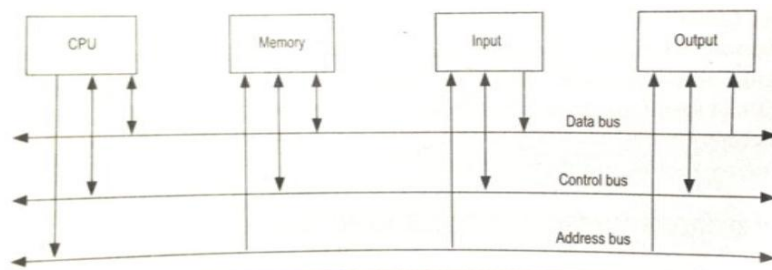
Fig.1 Microprocessor-based system
